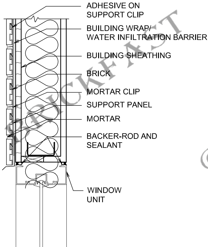
TYPICAL WINDOW DETAIL
