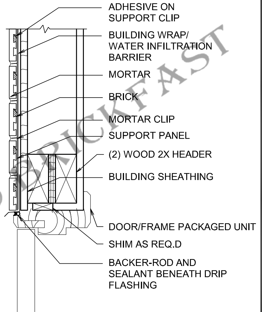
TYPICAL DOOR DETAIL
