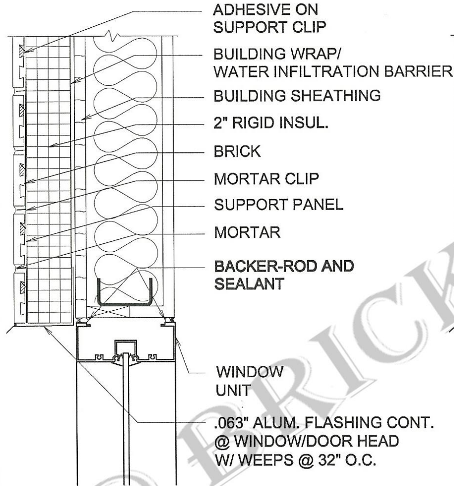
TYPICAL WINDOW DETAIL
